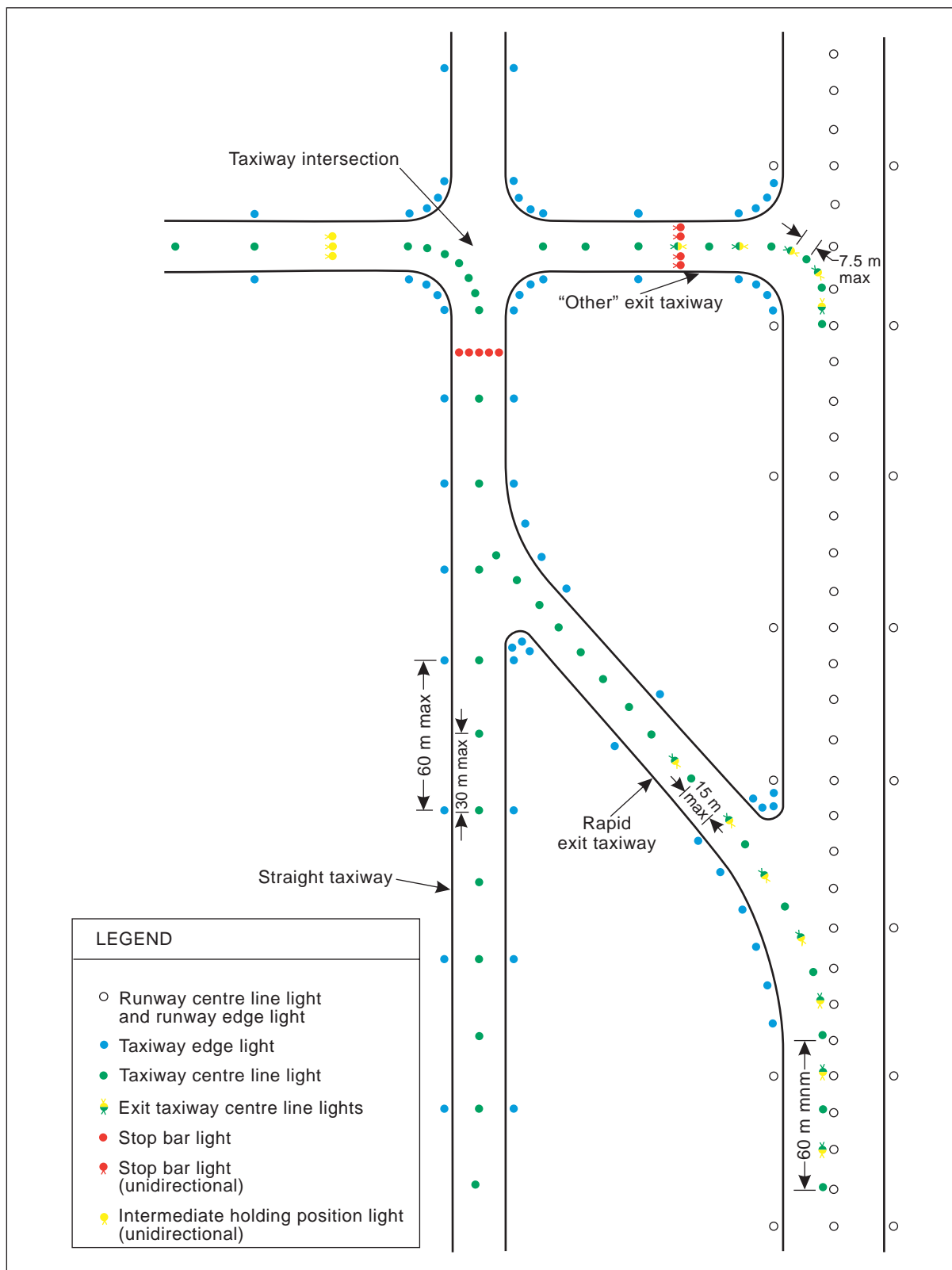
Figure 5-25. Taxiway lighting
