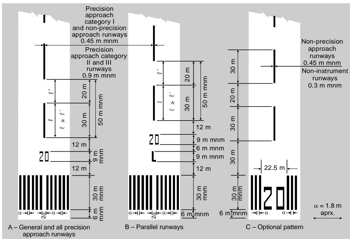
Figure 5-2. Runway designation, centre line and threshold markings
